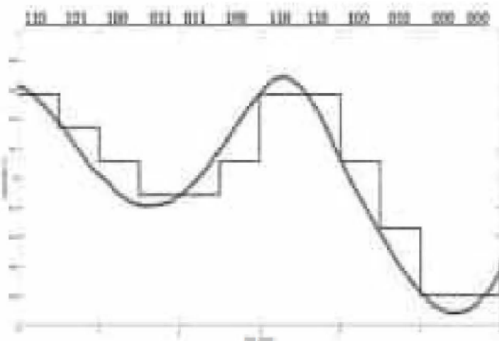
Fig: 14.19 Reconstruction of Analog Signal
